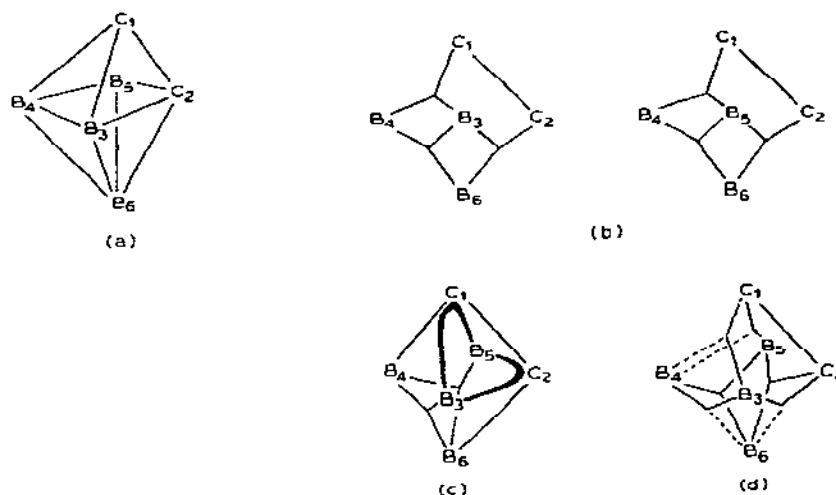
Fig. 19. Bonding in 1,2\text{-C}_2\text{B}_4\text{H}_6 . (a) The geometrical structure; (b) the localised molecular orbitals calculated by Guest and Hillier (ref. 240); (c) the localised molecular orbitals calculated by Lipscomb (ref. 250) using the Edmiston-Ruedenberg procedure; and (d) the localised molecular orbitals calculated by Lipscomb (ref. 250) using the Boys method.
