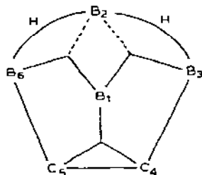
Fig. 22. The localised molecular orbitals for 4,5- C_2B_4H_8 .
