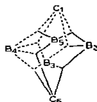
Fig. 20. The localised molecular orbitals for 1,6\text{-C}_2\text{B}_4\text{H}_6 .
