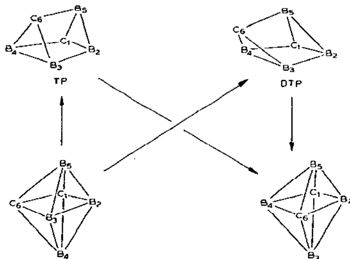
Fig. 21. The rearrangement schemes of 1,2- C_2B_4H_6 to 1,6- C_2B_4H_6 .
