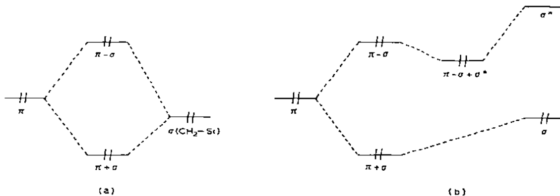
Fig. 38. Orbital diagrams of allylsilane: (a) in the absence of a \sigma^*(\text{CH}_2\text{-Si}) orbital and (b) in the presence of a low-lying \sigma^*(\text{CH}_2\text{-Si}) orbital.
