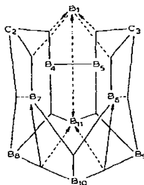
Fig. 28. The localised molecular orbitals for 1,6- C_2B_8H_{10} .
