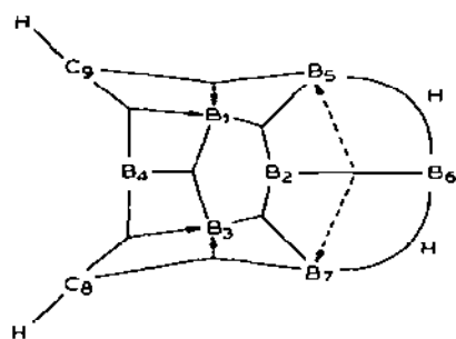
Fig. 27. The localised molecular orbitals for 8,9- C_2B_7H_{13} .
