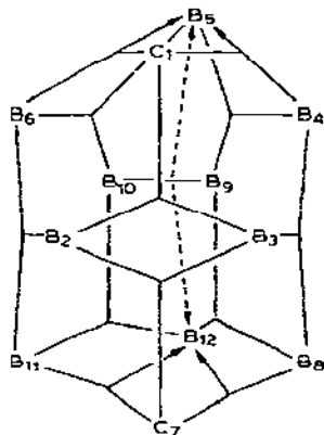
Fig. 32. The localised molecular orbitals for 1,7\text{-C}_2\text{B}_{10}\text{H}_{12} .
