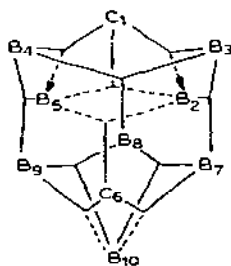
Fig. 28. The localised molecular orbitals for 1,6- C_2B_8H_{10} .
