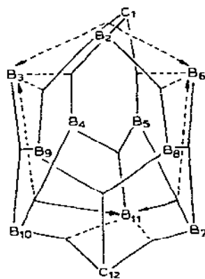
Fig. 32. The localised molecular orbitals for 1,7\text{-C}_2\text{B}_{10}\text{H}_{12} .
